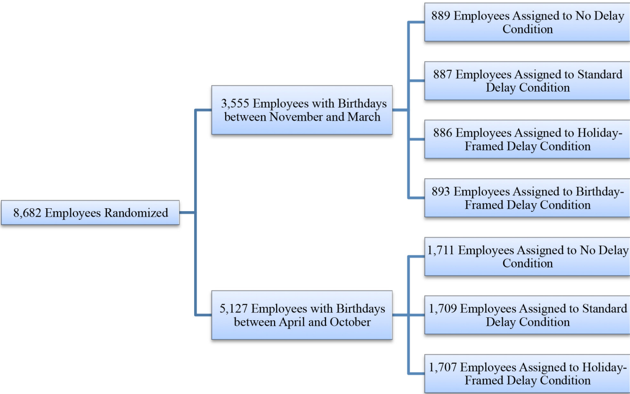
FIGURE 1. STUDY FLOW
