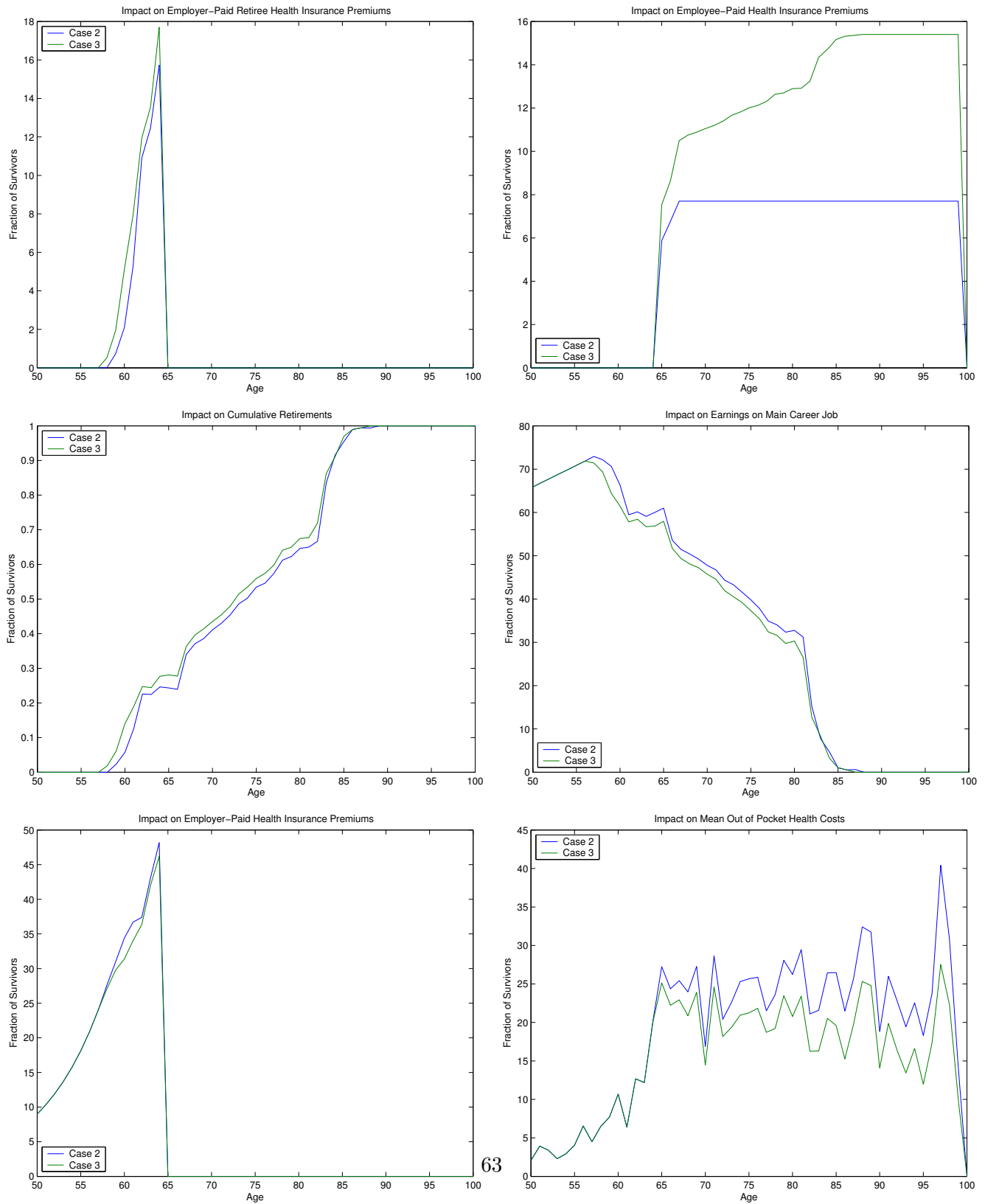
Figure 18: Comparisons of Case 2 and Case 3: Effects of Cancelling RHI after Age 65 with/without fairly priced Medigap coverage
