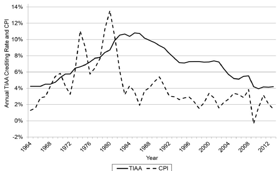
TIAA Average Crediting Rates Versus Consumer Price Index: 1964-2013
